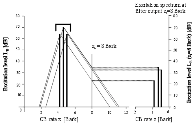
Figure 3: Excitation pattern for AM, slopes are calculated from the summation level.
