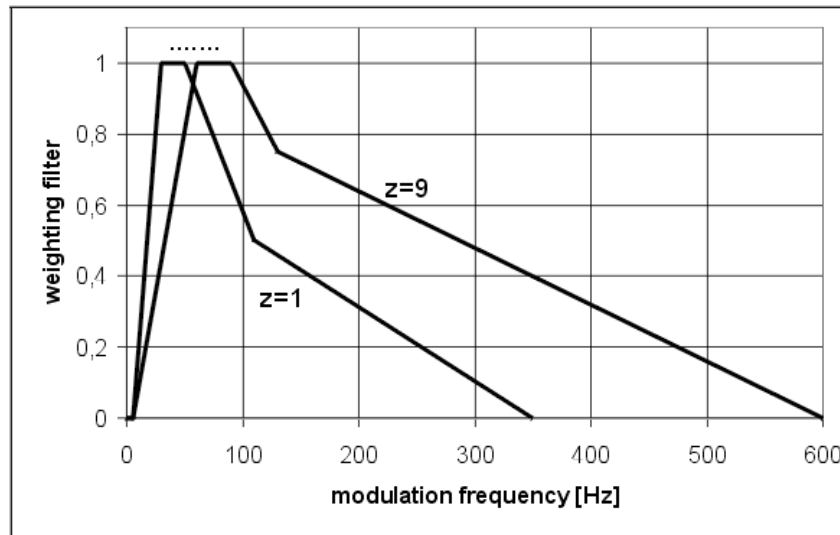
Figure 4: Bandpass weighting filters as proposed in [5]
