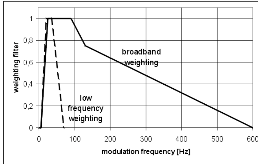
Figure 5: Frequency independent weighting filters
