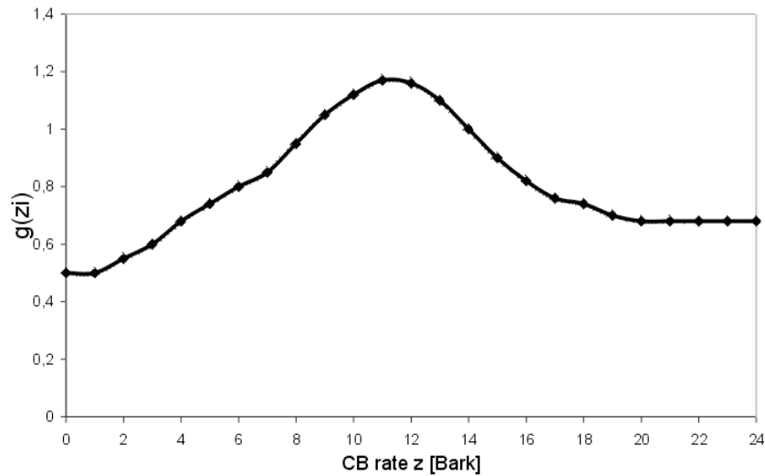
Figure 6: Weighting function g(z_i) for carrier frequency according to [4]
