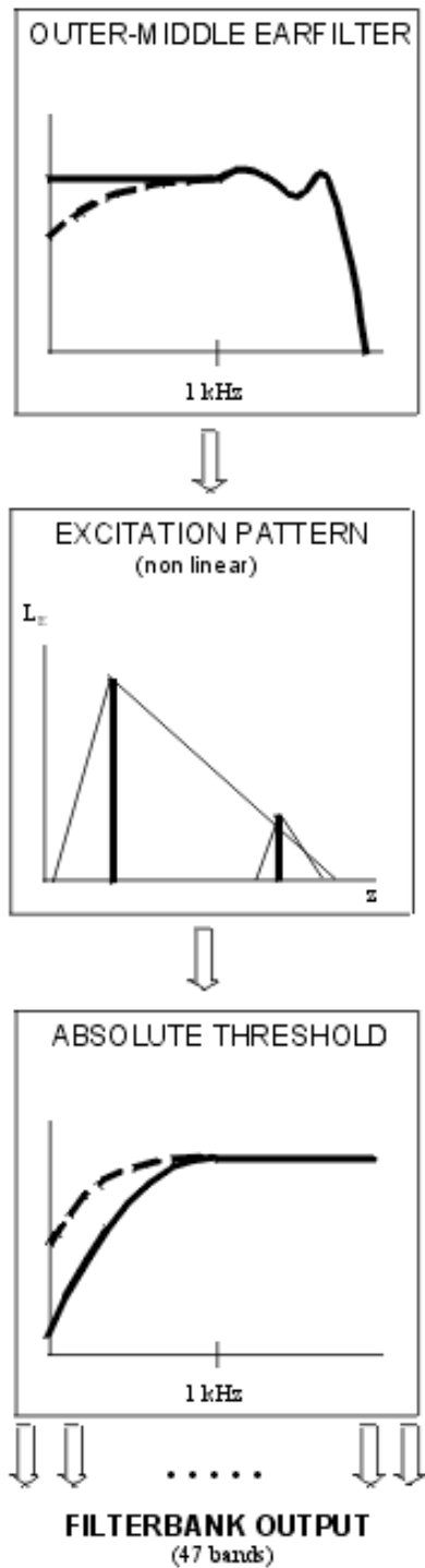
Figure 1: Calculation scheme of the excitation pattern
